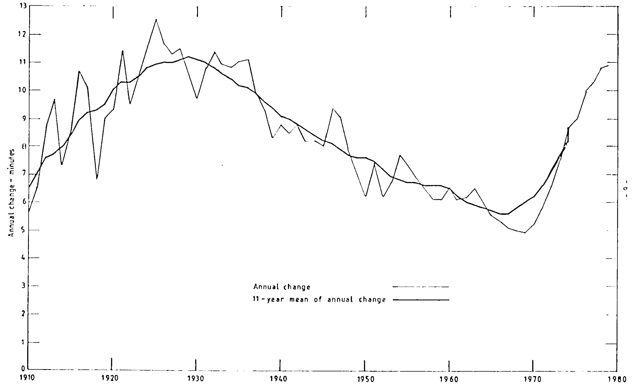
Fig. 2. Annual change in declination at Valentia.
